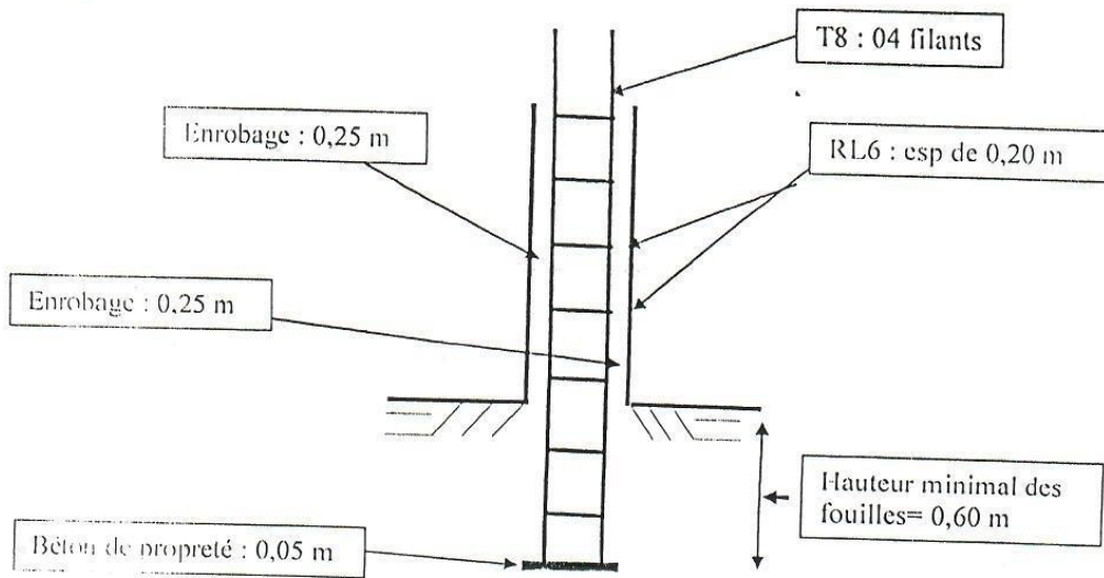
Ferraillage Amorce poteau
