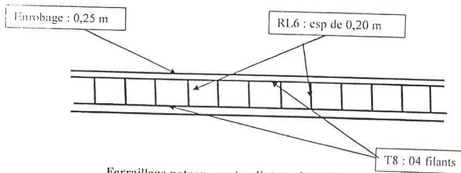
Ferraillage poteau, poutre, linteau, longrine
